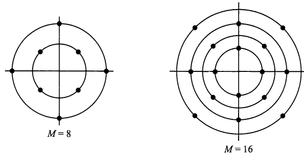
Figure 21: Examples of combined PAM-PSK constellations.
