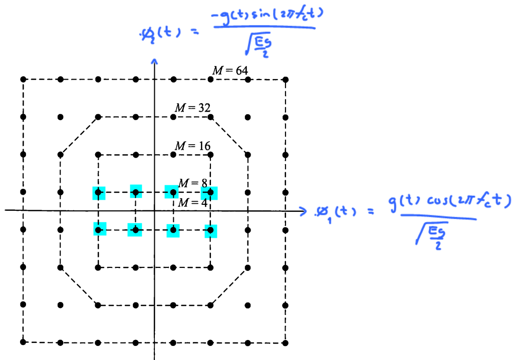
Figure 22: Several signal space diagrams for rectangular QAM.
