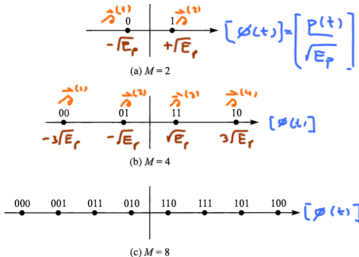
Figure 19: Constellation for PAM signaling
