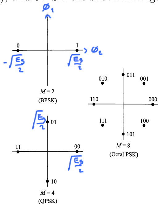
Figure 20: Signal space diagrams for BPSK, QPSK, and 8-PSK.
