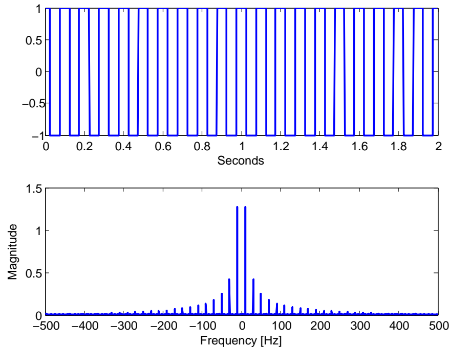
Figure 9.1: Plots from specsquare.m
