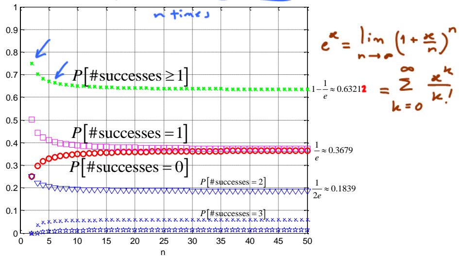
Figure 10: Number of occurrences of 1-in- n -chance event in n repeated Bernoulli trials
